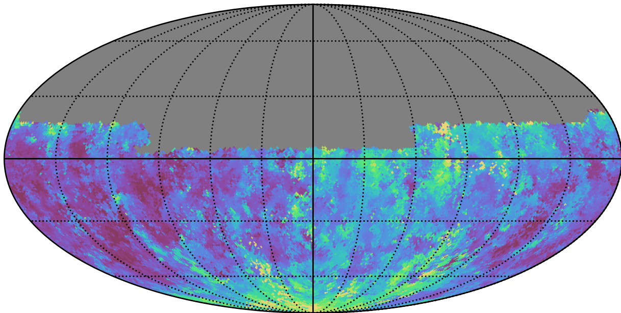
extra_ss_neo3_v3.4_10yrs Yr 1 u band: Median seeingEff
