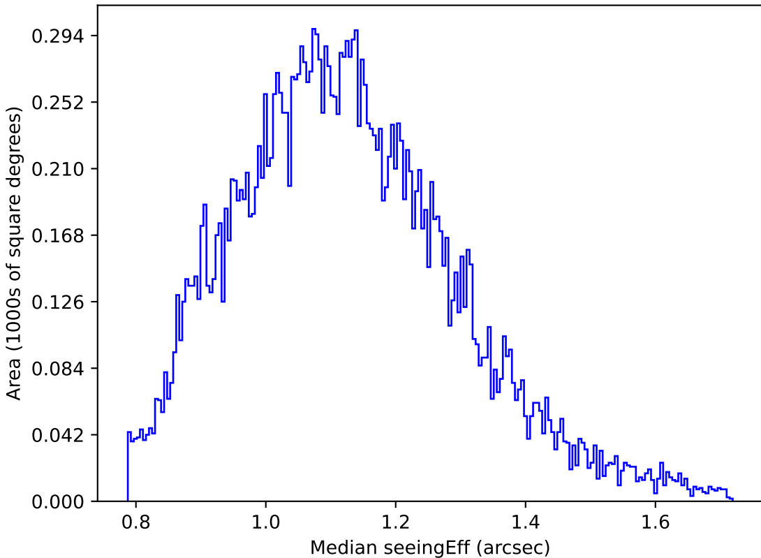
extra_ss_neo3_v3.4_10yrs Yr 1 u band: Median seeingEff
