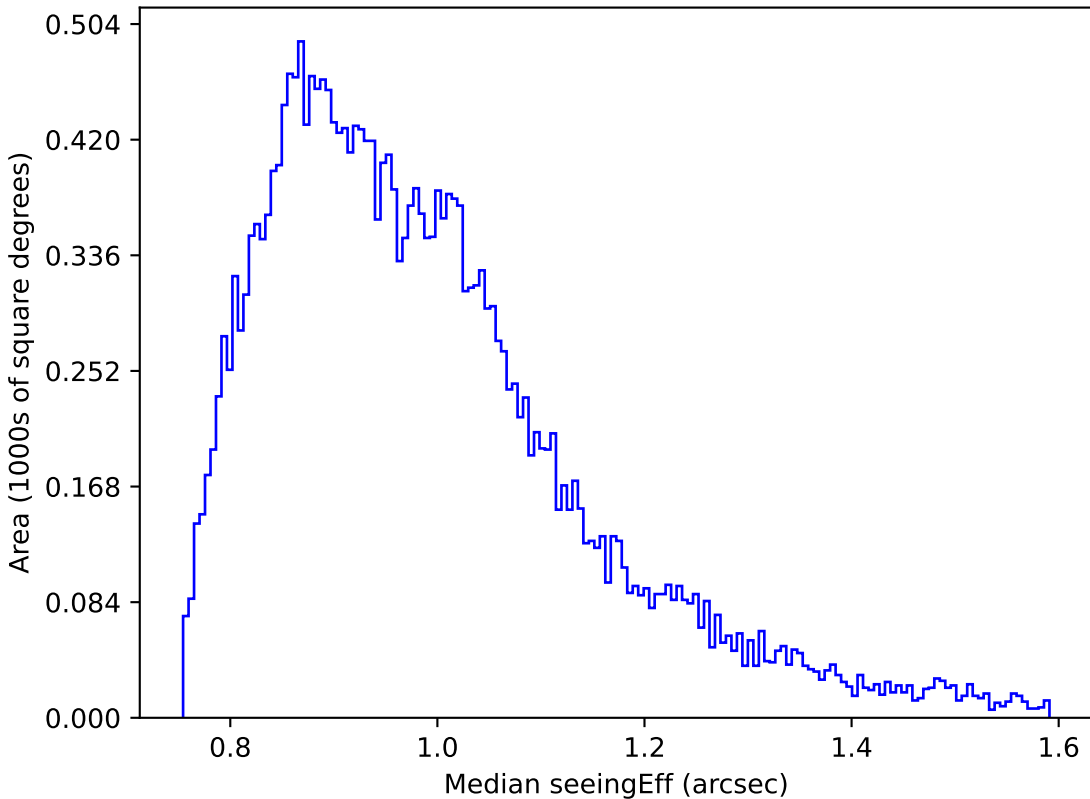
extra_ss_neo3_v3.4_10yrs Yr 1 r band: Median seeingEff
