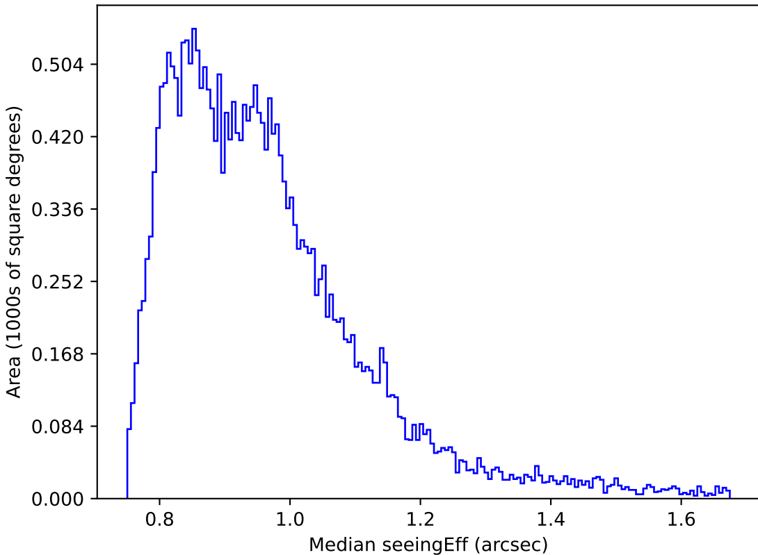
extra_ss_neo3_v3.4_10yrs Yr 1 i band: Median seeingEff
