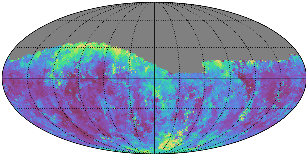
extra_ss_neo3_v3.4_10yrs Yr 1 g band: Median seeingEff
