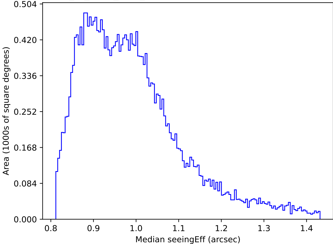
extra_ss_neo3_v3.4_10yrs Yr 1 all bands: Median seeingEff
