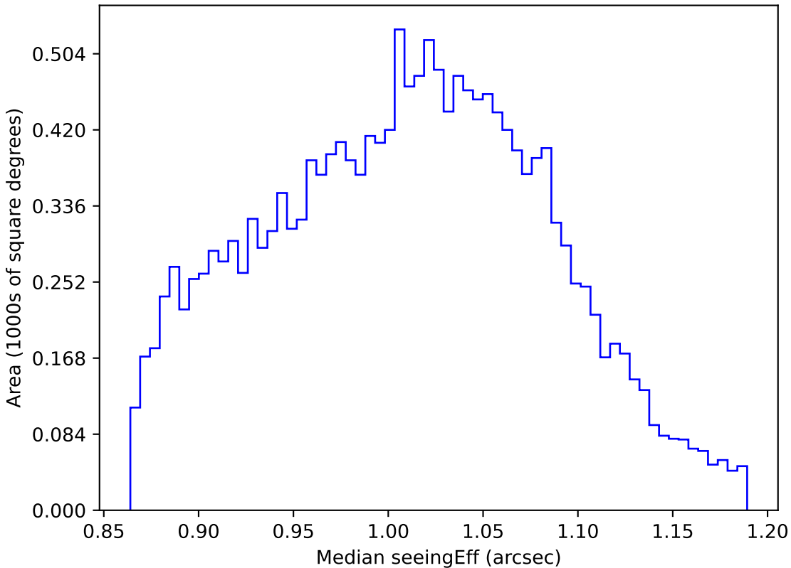
extra_ss_neo3_v3.4_10yrs WFD z band: Median seeingEff
