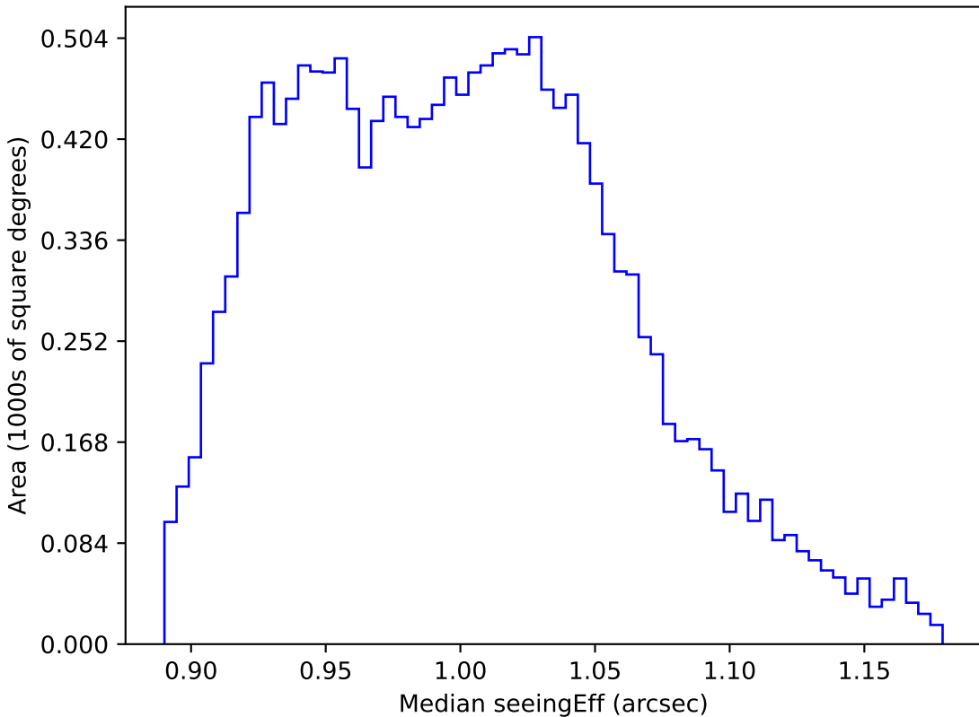
extra_ss_neo3_v3.4_10yrs WFD y band: Median seeingEff
