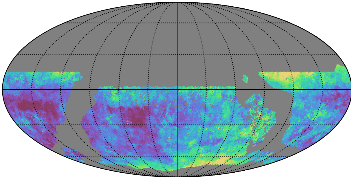
extra_ss_neo3_v3.4_10yrs WFD u band: Median seeingEff
