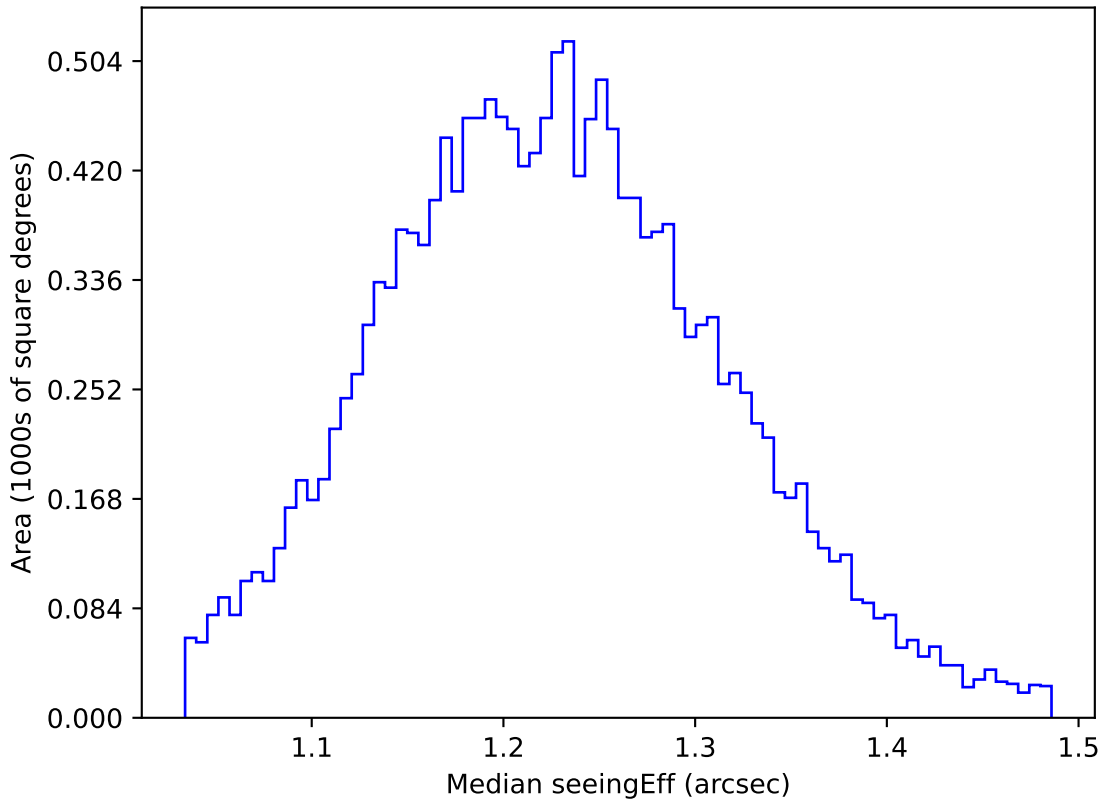
extra_ss_neo3_v3.4_10yrs WFD u band: Median seeingEff
