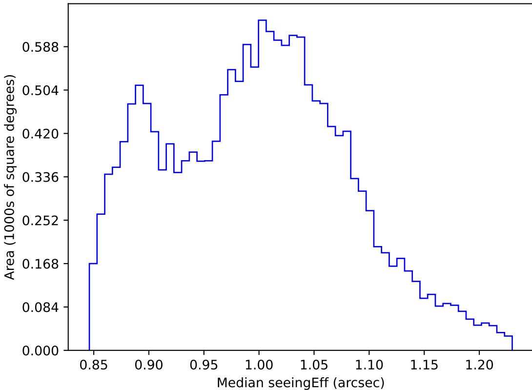
extra_ss_neo3_v3.4_10yrs WFD i band: Median seeingEff
