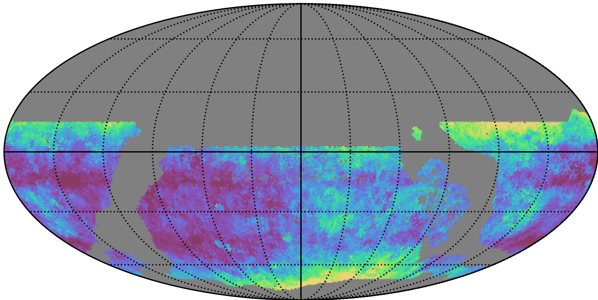
extra_ss_neo3_v3.4_10yrs WFD g band: Median seeingEff
