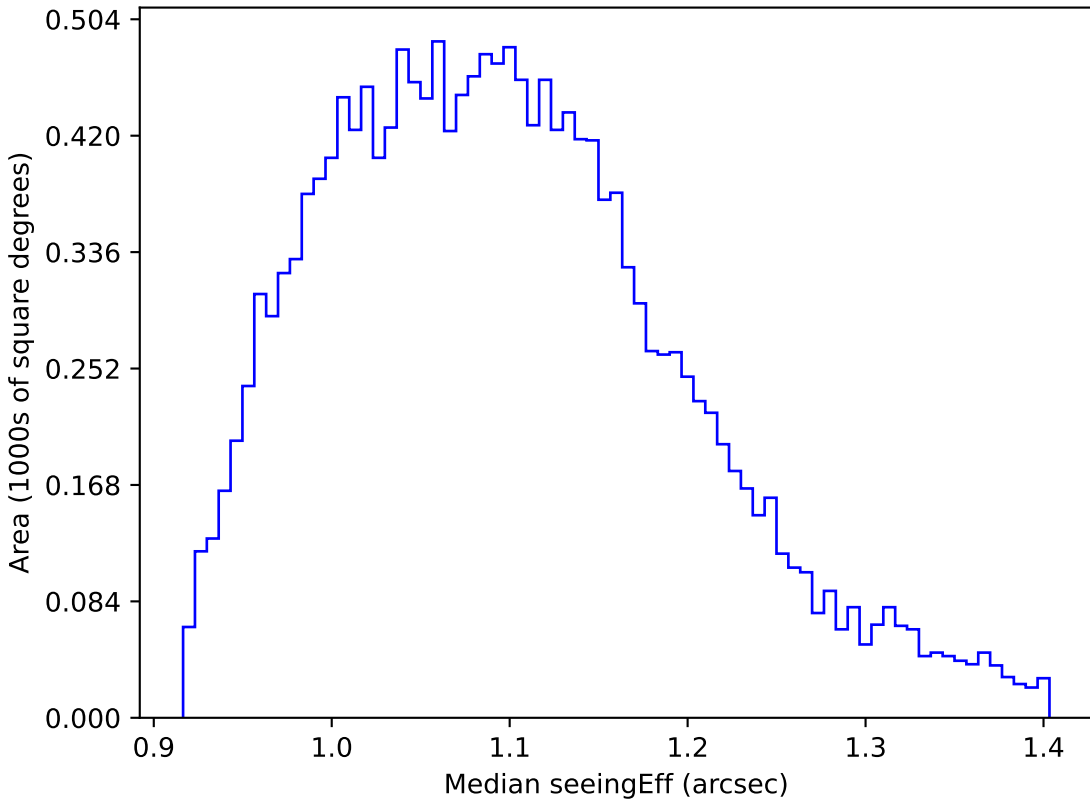
extra_ss_neo3_v3.4_10yrs WFD g band: Median seeingEff
