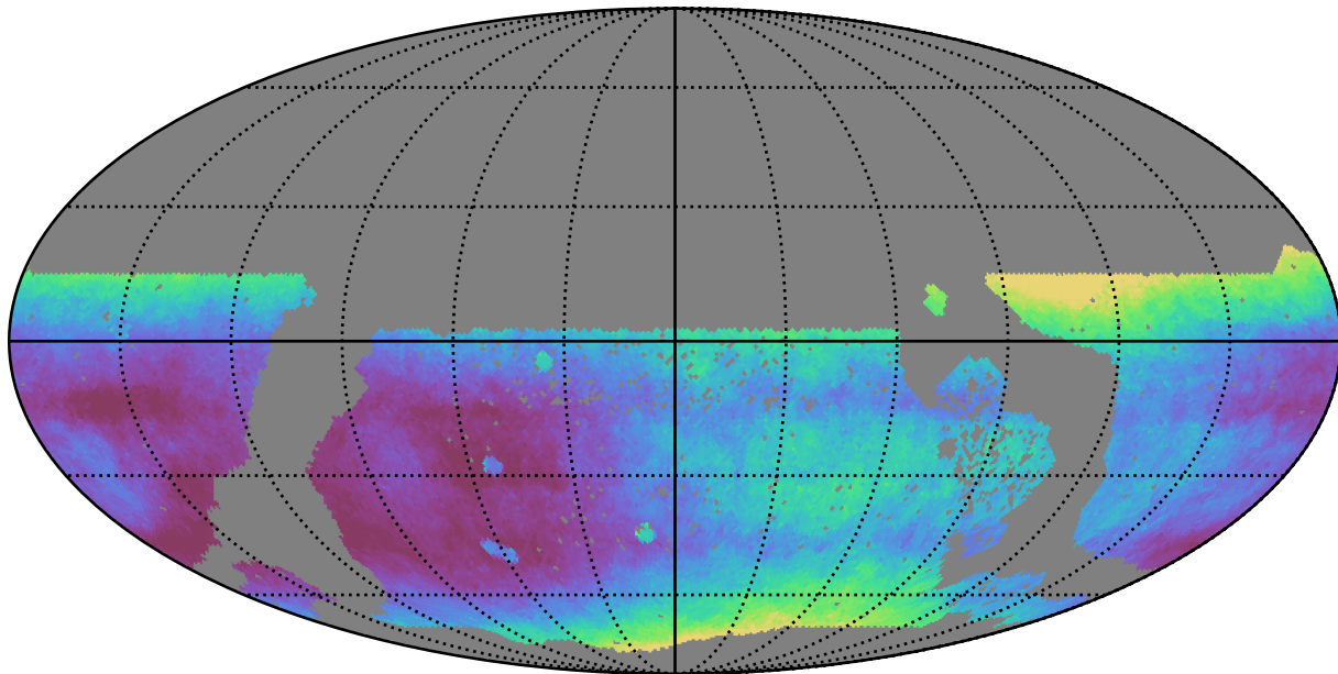
extra_ss_neo3_v3.4_10yrs WFD all bands: Median seeingEff
