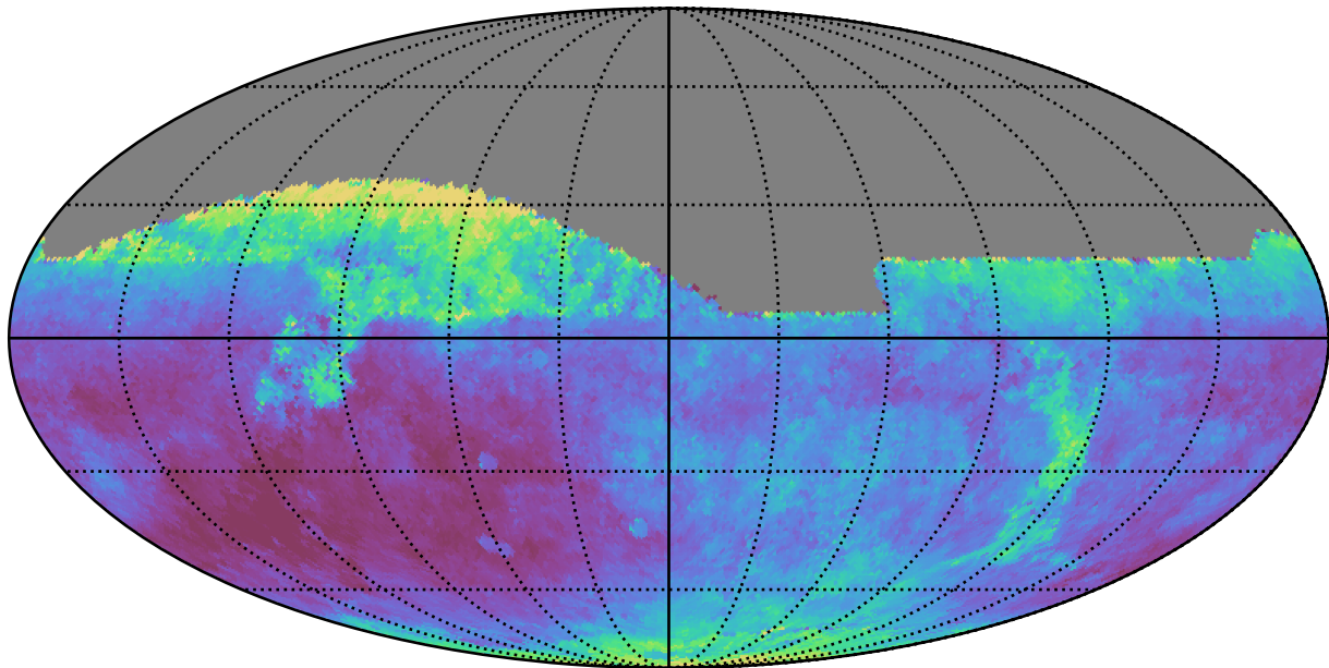
extra_ss_neo3_v3.4_10yrs All sky z band: Median seeingEff
