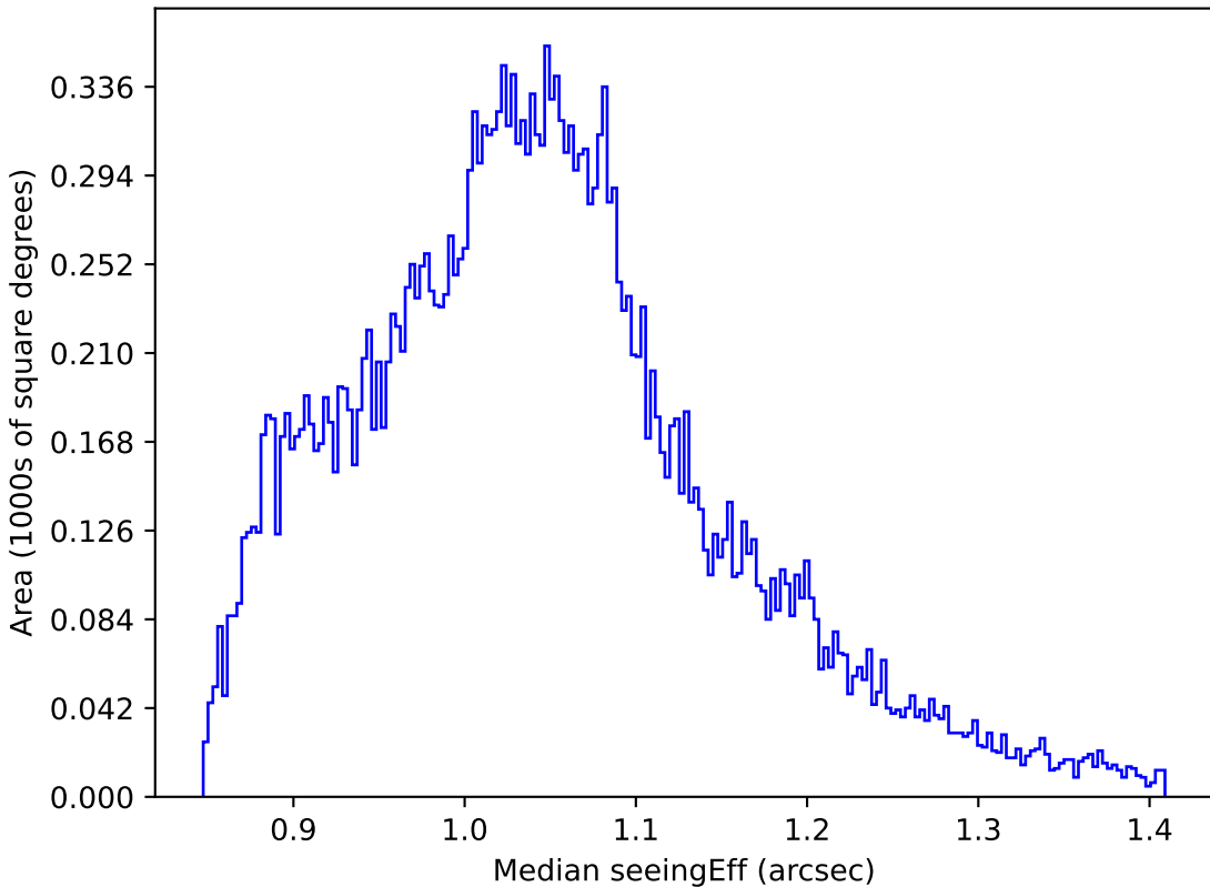
extra_ss_neo3_v3.4_10yrs All sky z band: Median seeingEff
