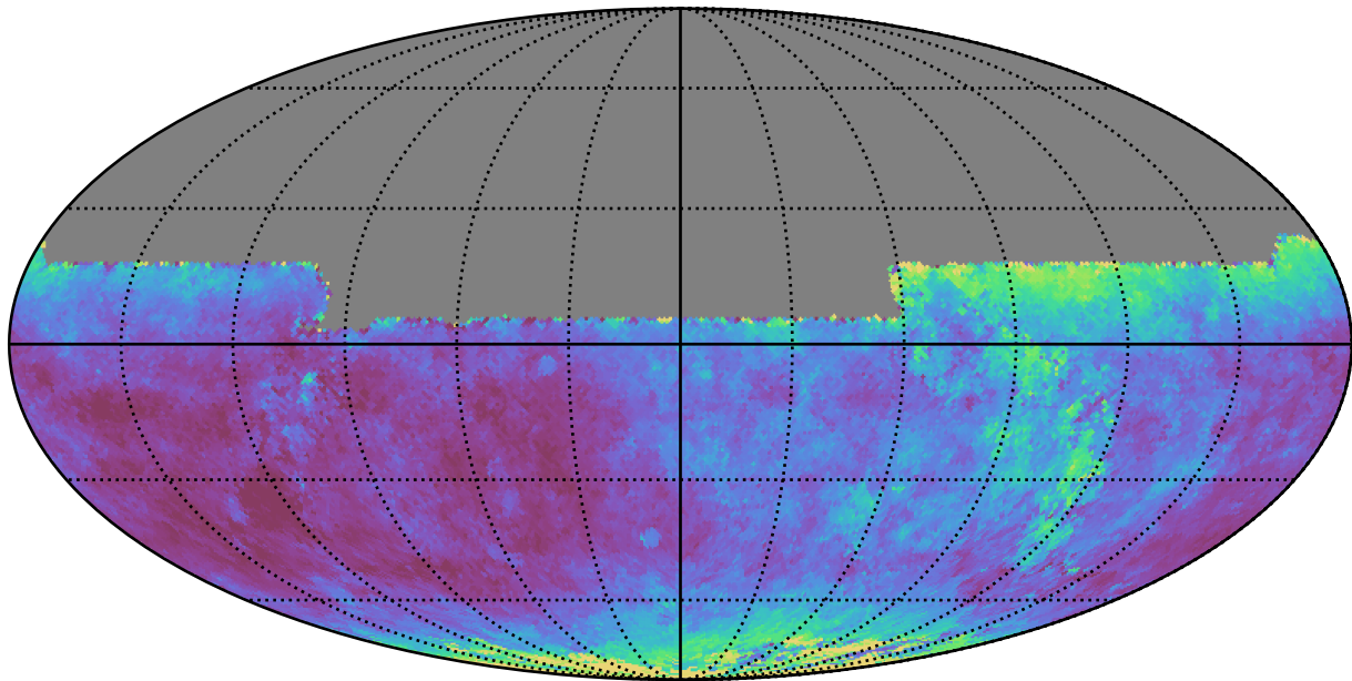
extra_ss_neo3_v3.4_10yrs All sky y band: Median seeingEff
