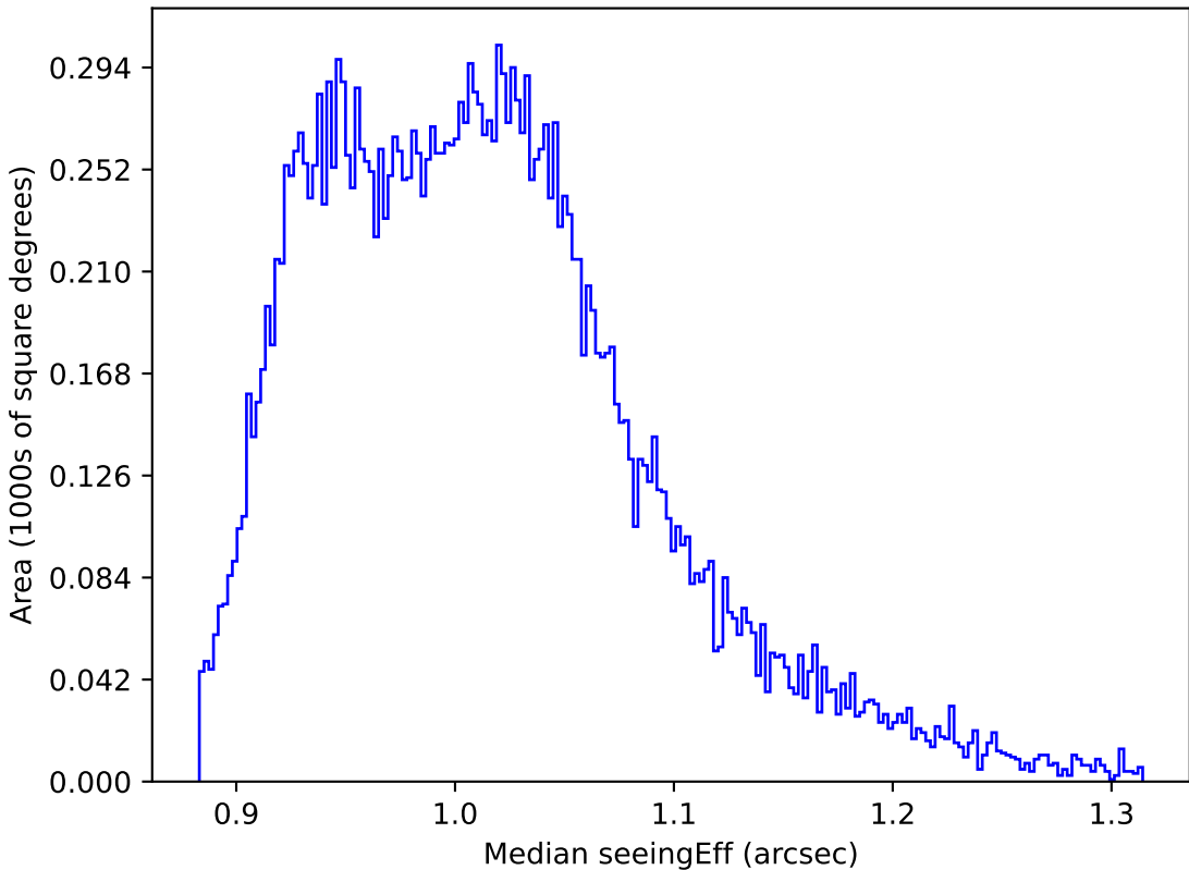
extra_ss_neo3_v3.4_10yrs All sky y band: Median seeingEff
