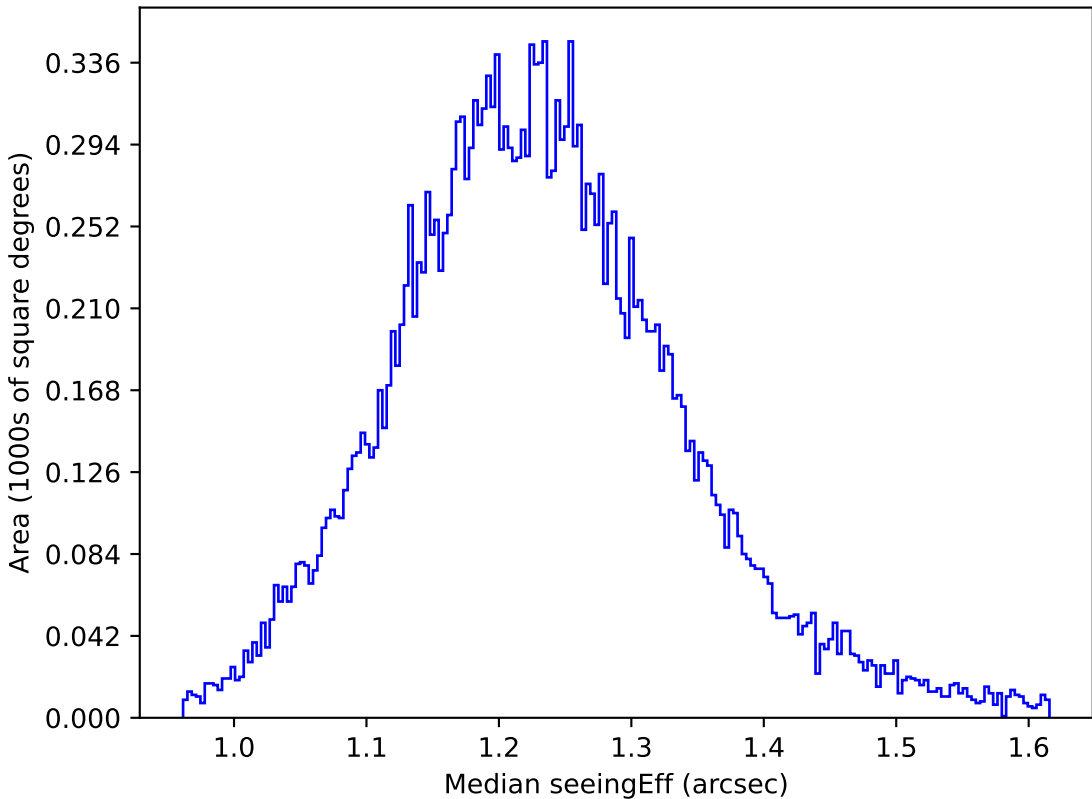
extra_ss_neo3_v3.4_10yrs All sky u band: Median seeingEff
