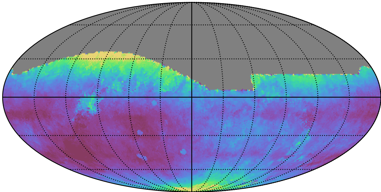
extra_ss_neo3_v3.4_10yrs All sky r band: Median seeingEff
