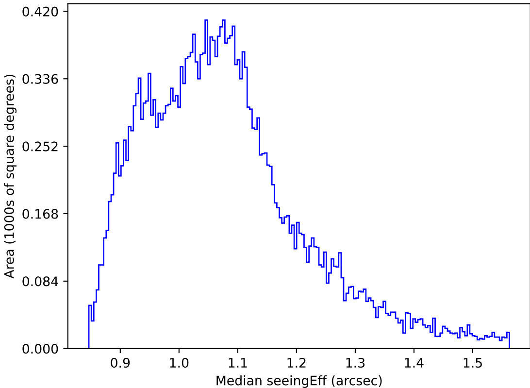
extra_ss_neo3_v3.4_10yrs All sky r band: Median seeingEff
