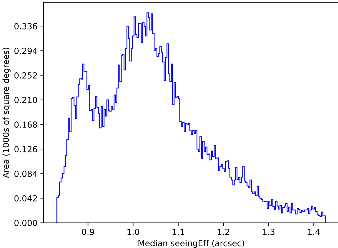
extra_ss_neo3_v3.4_10yrs All sky i band: Median seeingEff
