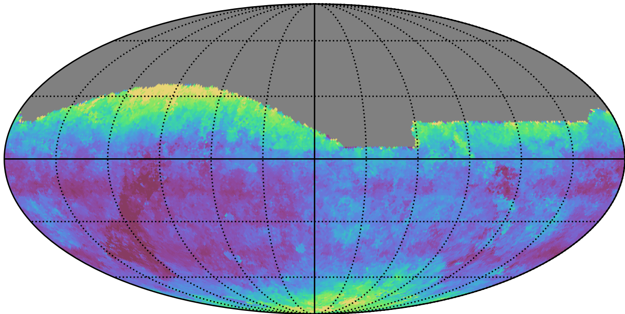
extra_ss_neo3_v3.4_10yrs All sky g band: Median seeingEff
