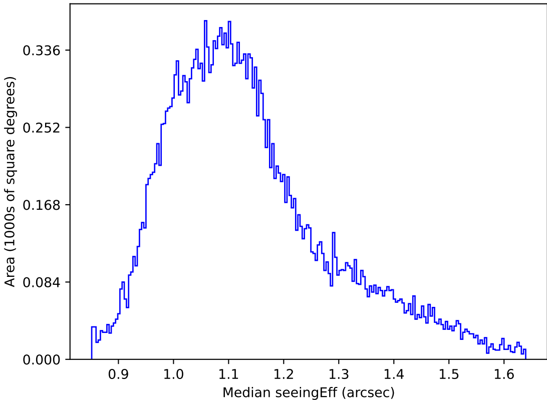
extra_ss_neo3_v3.4_10yrs All sky g band: Median seeingEff
