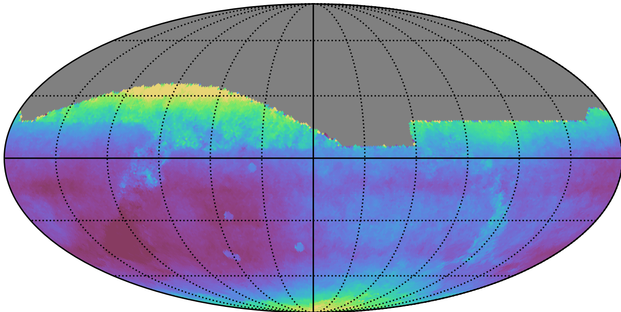
extra_ss_neo3_v3.4_10yrs All sky all bands: Median seeingEff
