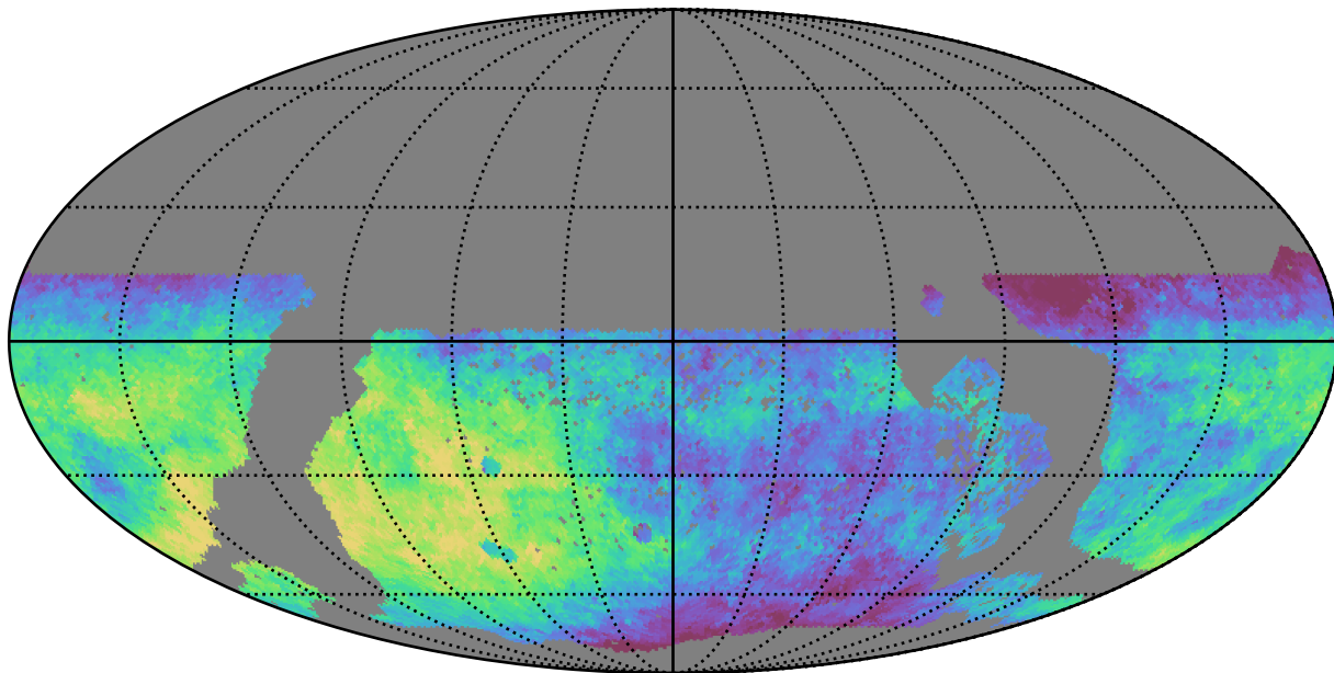
extra_ss_neo3_v3.4_10yrs WFD z band: Median saturation_mag
