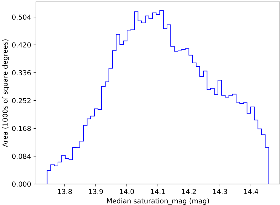
extra_ss_neo3_v3.4_10yrs WFD z band: Median saturation_mag
