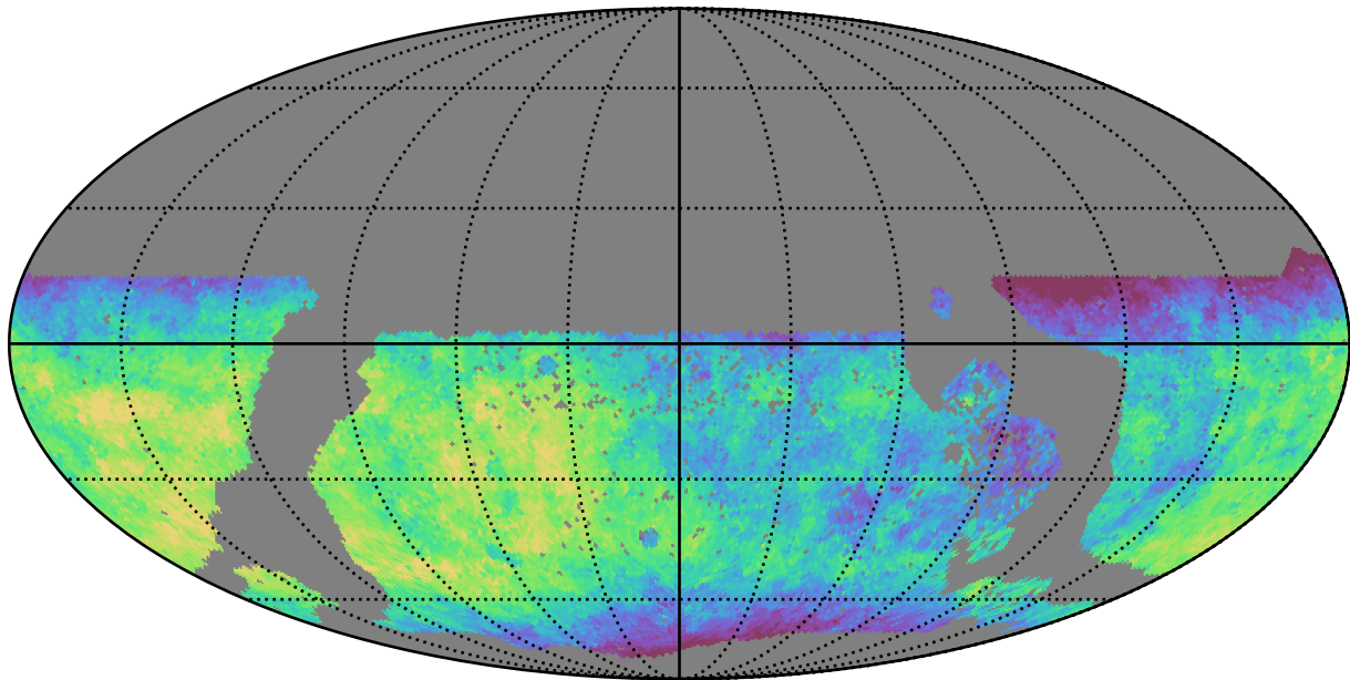
extra_ss_neo3_v3.4_10yrs WFD y band: Median saturation_mag
