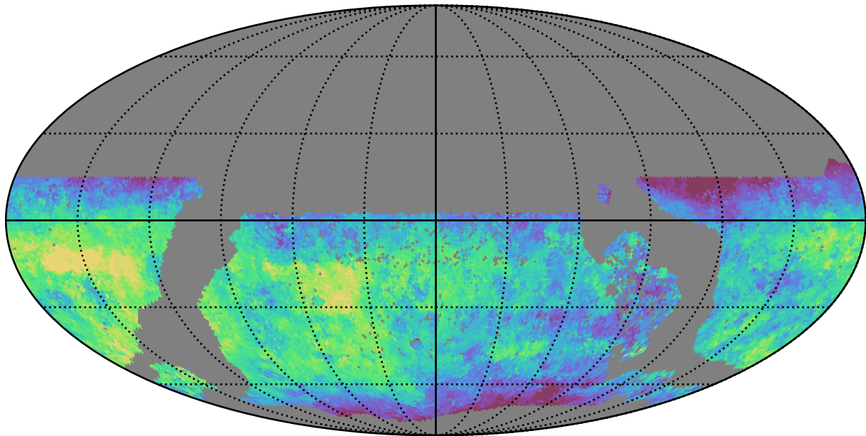
extra_ss_neo3_v3.4_10yrs WFD u band: Median saturation_mag
