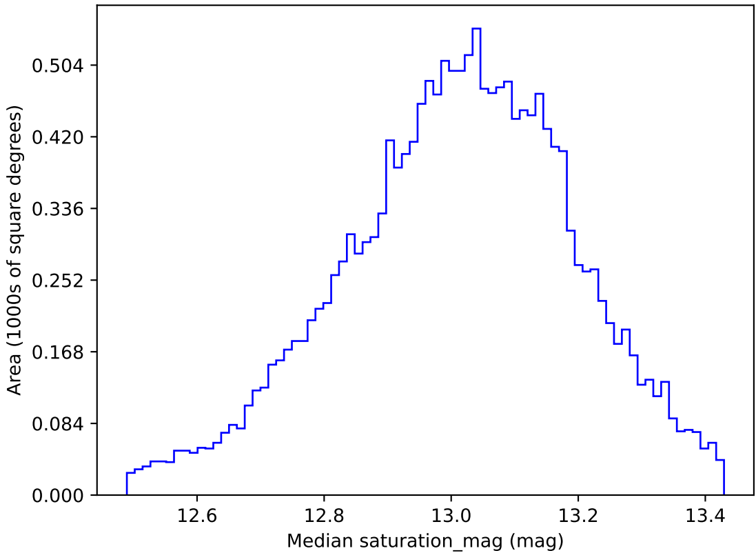
extra_ss_neo3_v3.4_10yrs WFD u band: Median saturation_mag
