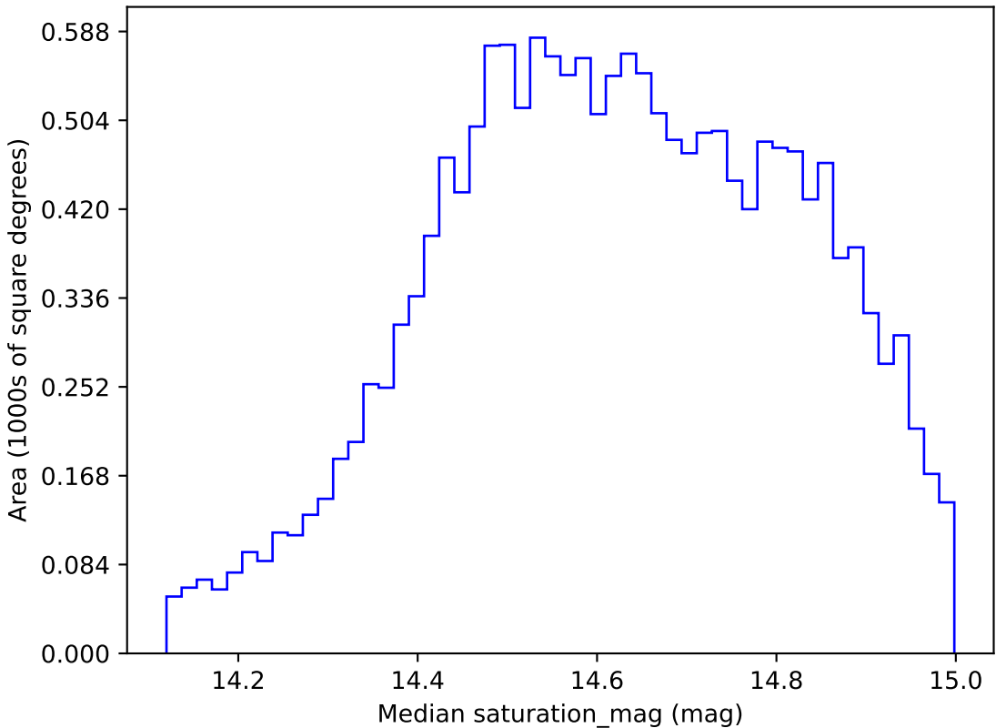
extra_ss_neo3_v3.4_10yrs WFD r band: Median saturation_mag
