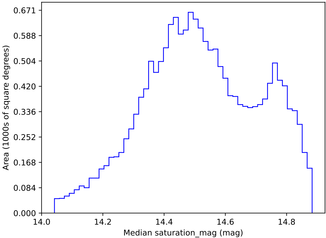
extra_ss_neo3_v3.4_10yrs WFD i band: Median saturation_mag
