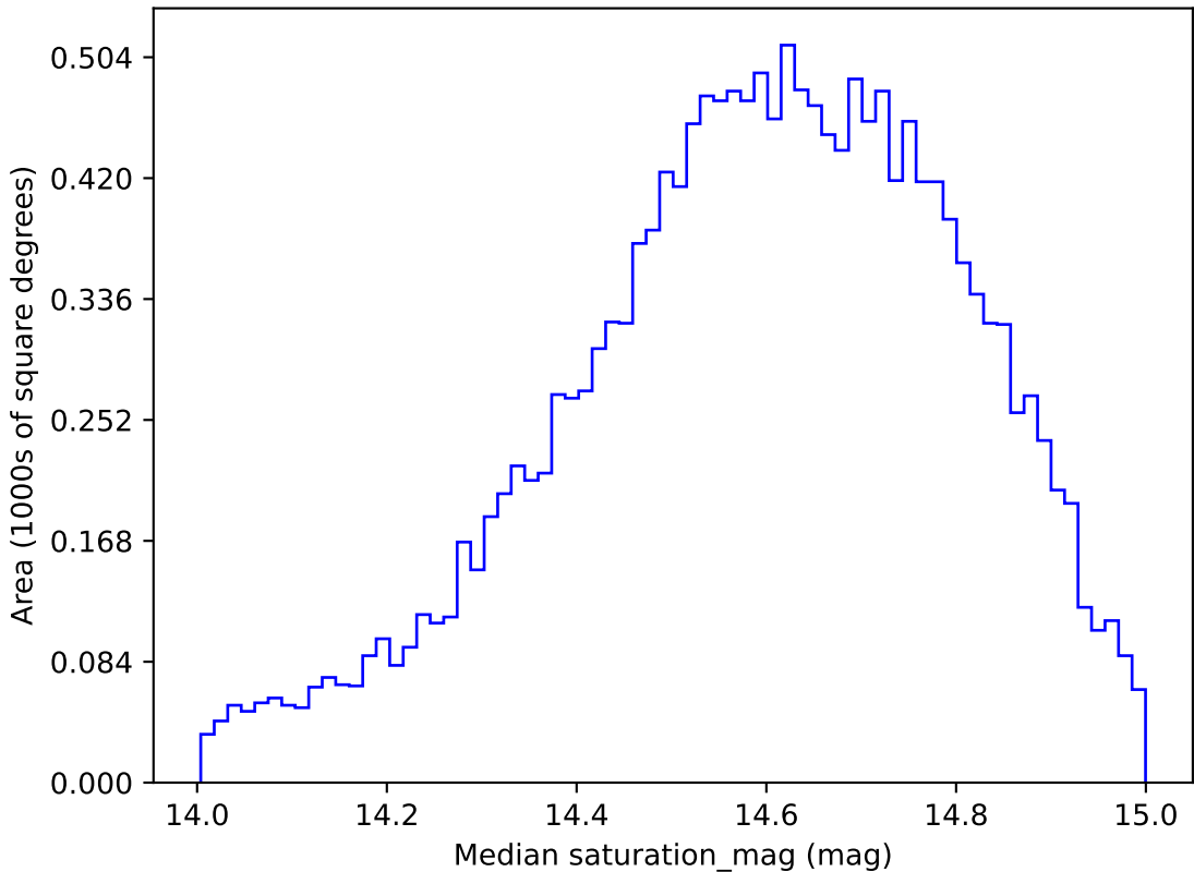
extra_ss_neo3_v3.4_10yrs WFD g band: Median saturation_mag
