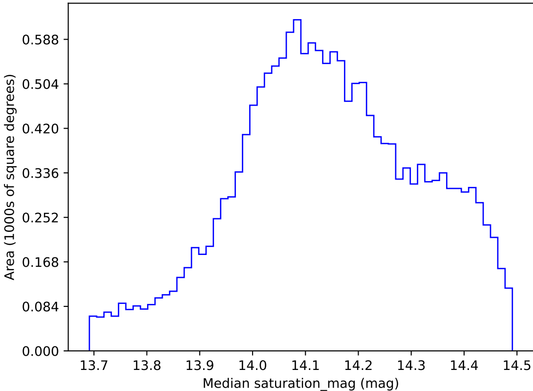
extra_ss_neo3_v3.4_10yrs WFD all bands: Median saturation_mag
