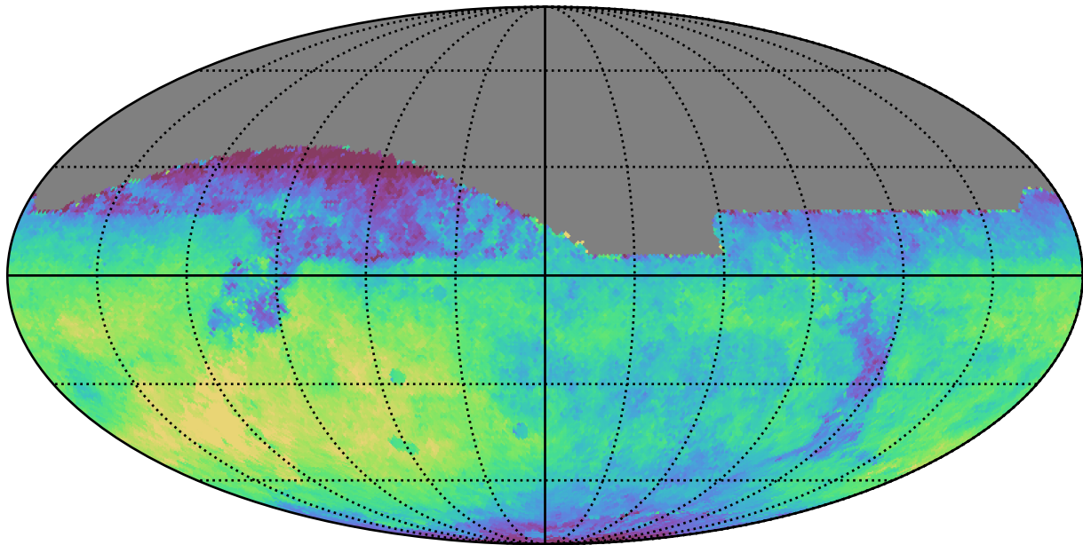
extra_ss_neo3_v3.4_10yrs All sky z band: Median saturation_mag
