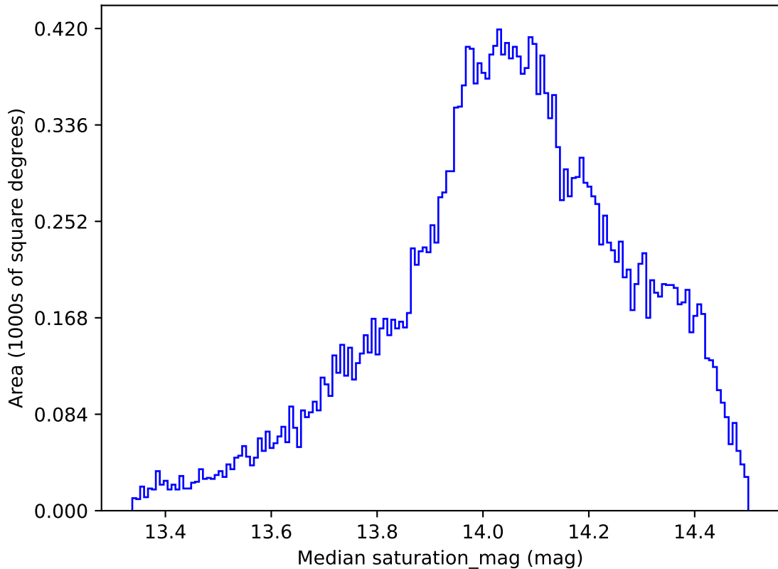
extra_ss_neo3_v3.4_10yrs All sky z band: Median saturation_mag
