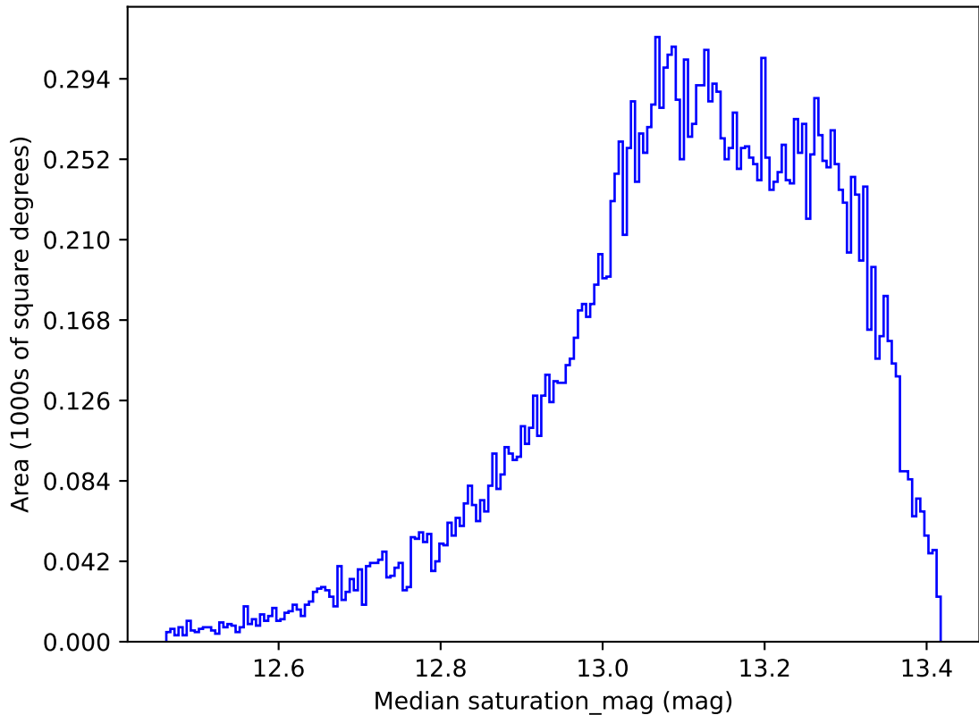
extra_ss_neo3_v3.4_10yrs All sky y band: Median saturation_mag
