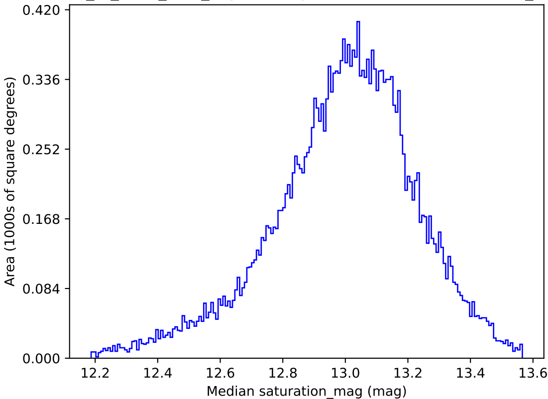
extra_ss_neo3_v3.4_10yrs All sky u band: Median saturation_mag
