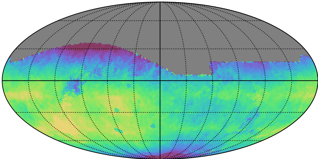
extra_ss_neo3_v3.4_10yrs All sky r band: Median saturation_mag
