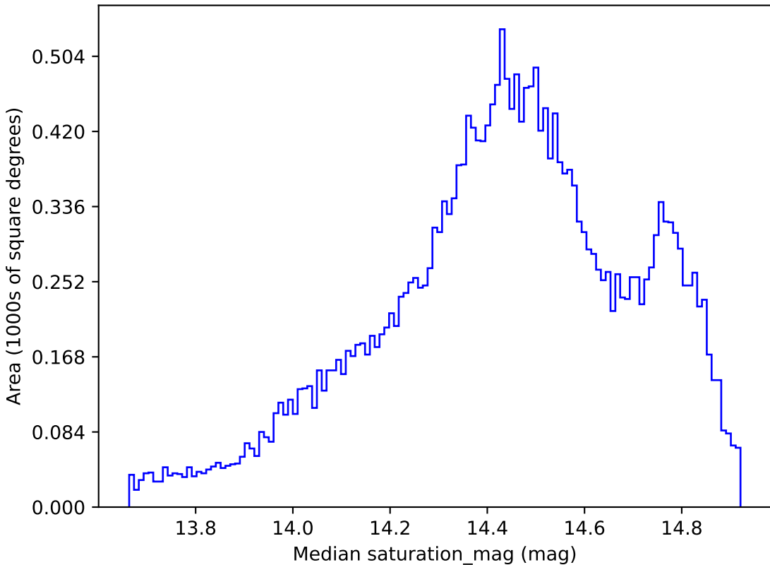
extra_ss_neo3_v3.4_10yrs All sky i band: Median saturation_mag
