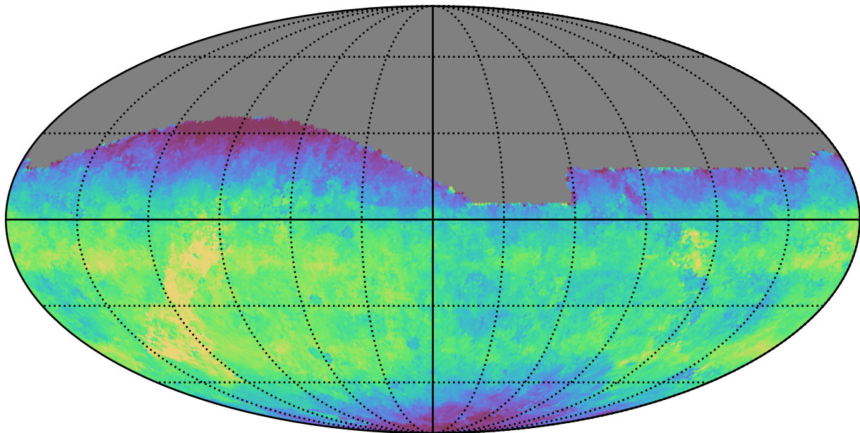
extra_ss_neo3_v3.4_10yrs All sky g band: Median saturation_mag
