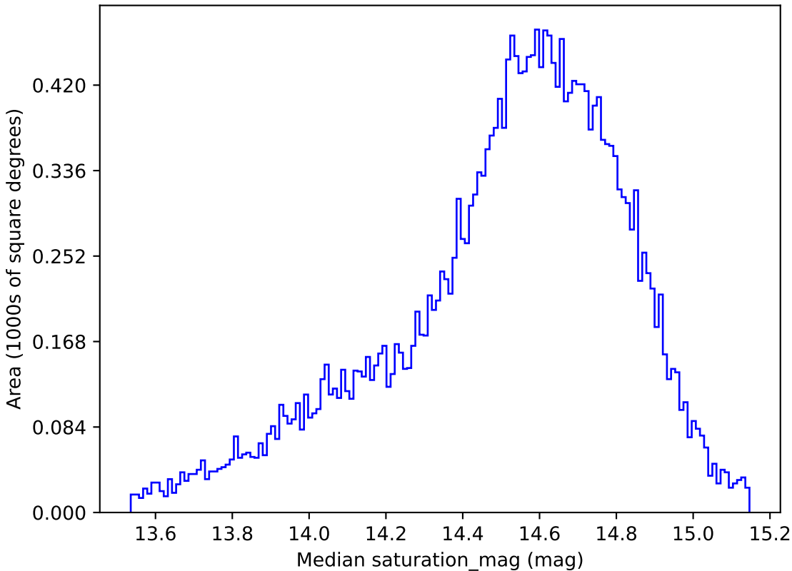
extra_ss_neo3_v3.4_10yrs All sky g band: Median saturation_mag
