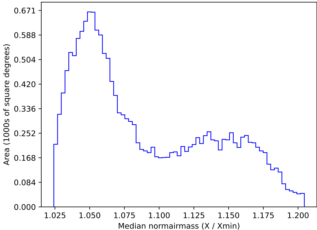
extra_ss_neo3_v3.4_10yrs WFD z band: Median normairmass
