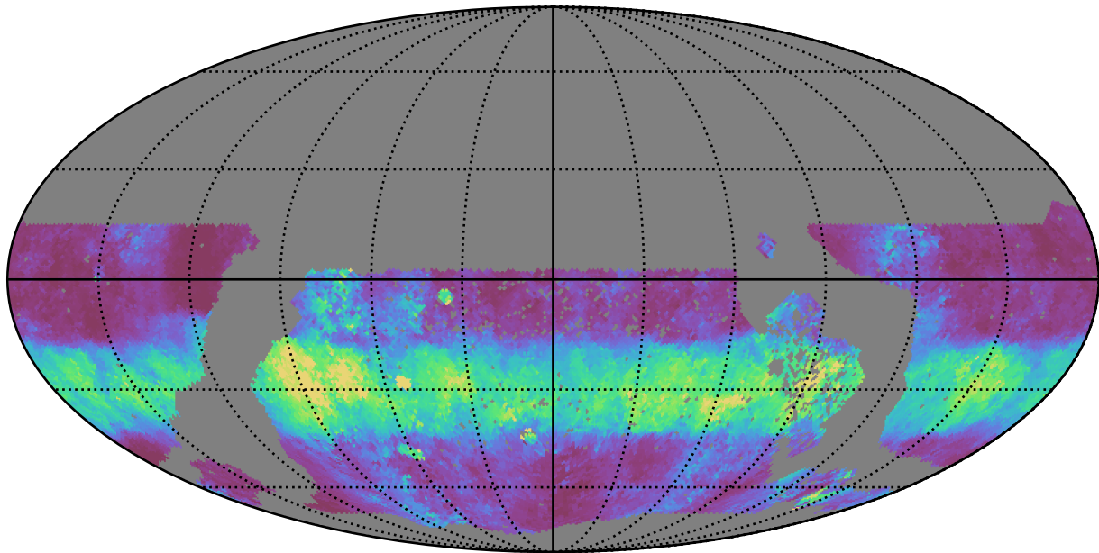
extra_ss_neo3_v3.4_10yrs WFD u band: Median normairmass
