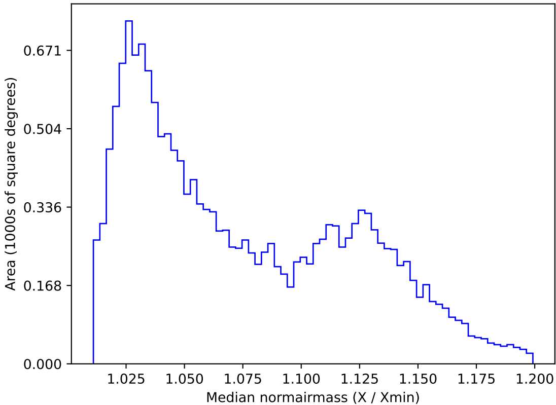
extra_ss_neo3_v3.4_10yrs WFD u band: Median normairmass
