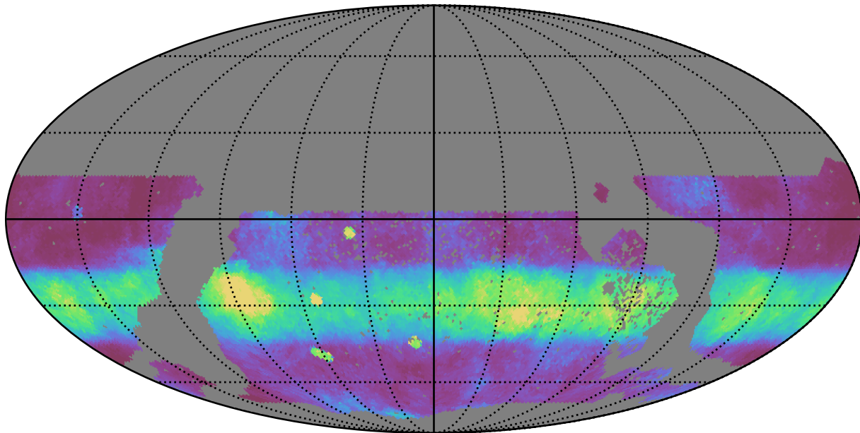
extra_ss_neo3_v3.4_10yrs WFD r band: Median normairmass
