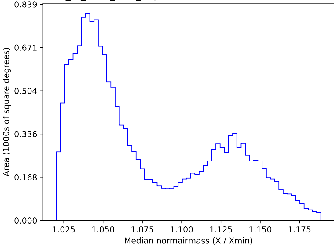
extra_ss_neo3_v3.4_10yrs WFD i band: Median normairmass
