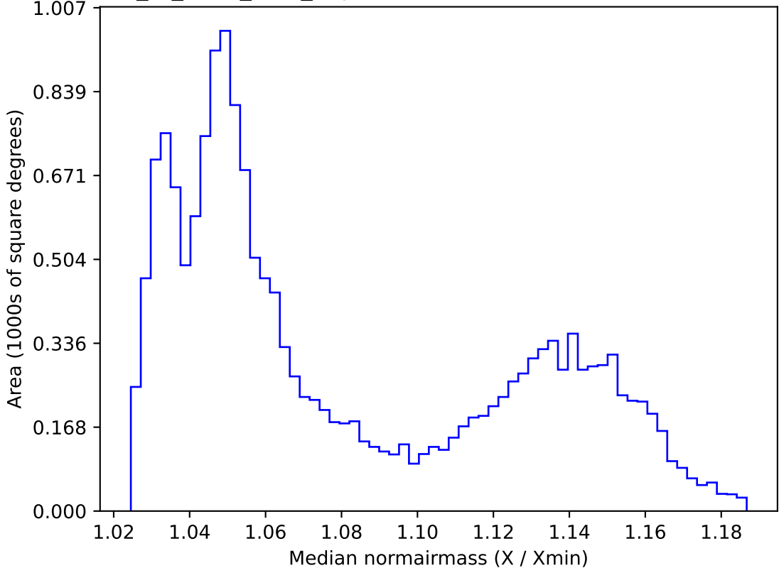
extra_ss_neo3_v3.4_10yrs WFD all bands: Median normairmass
