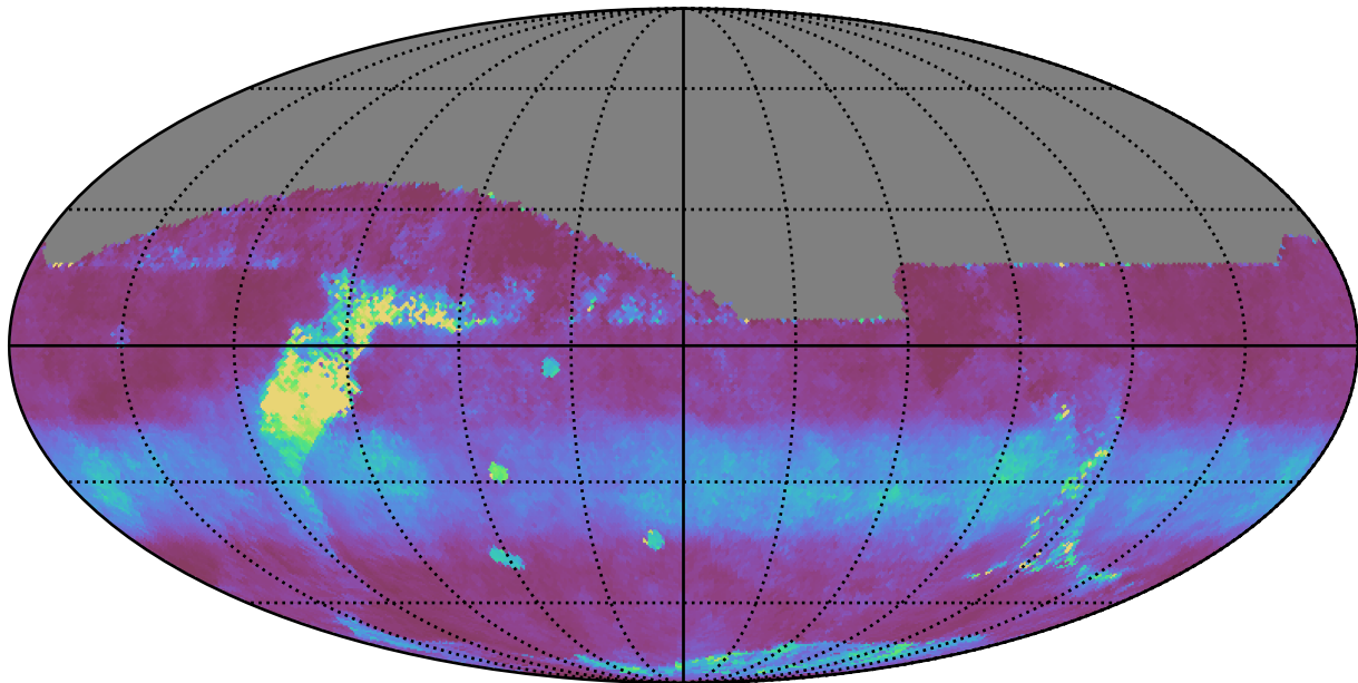
extra_ss_neo3_v3.4_10yrs All sky z band: Median normairmass
