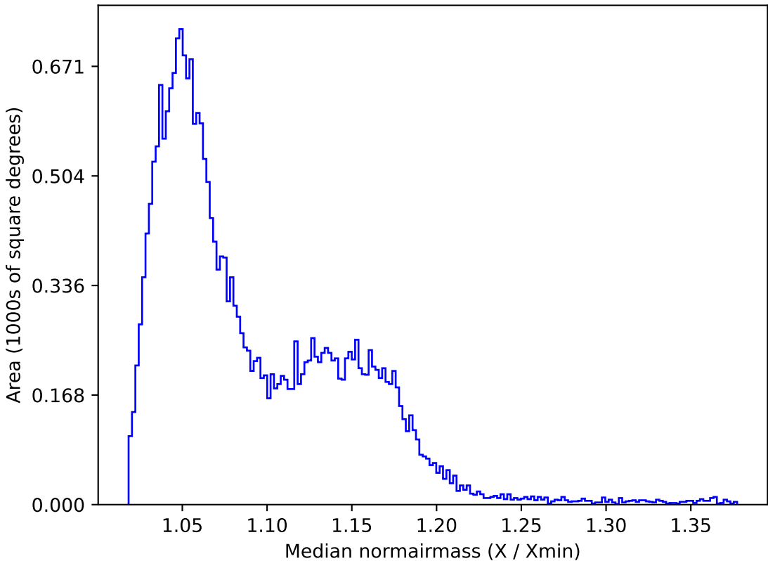
extra_ss_neo3_v3.4_10yrs All sky z band: Median normairmass
